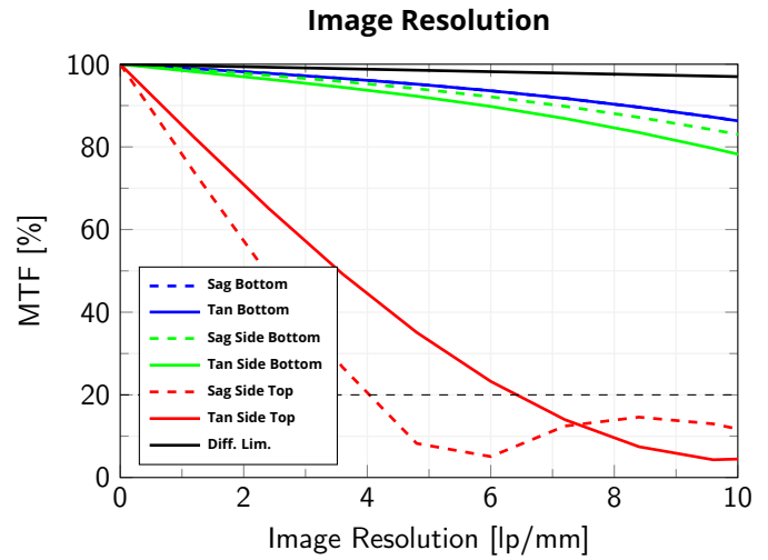
Modulation Transfer Function (MTF) vs. Image Resolution, wavelength range 486 nm - 656 nm of cylindrical object of diameter 50 mm and height of 150 mm at wf/N=4
